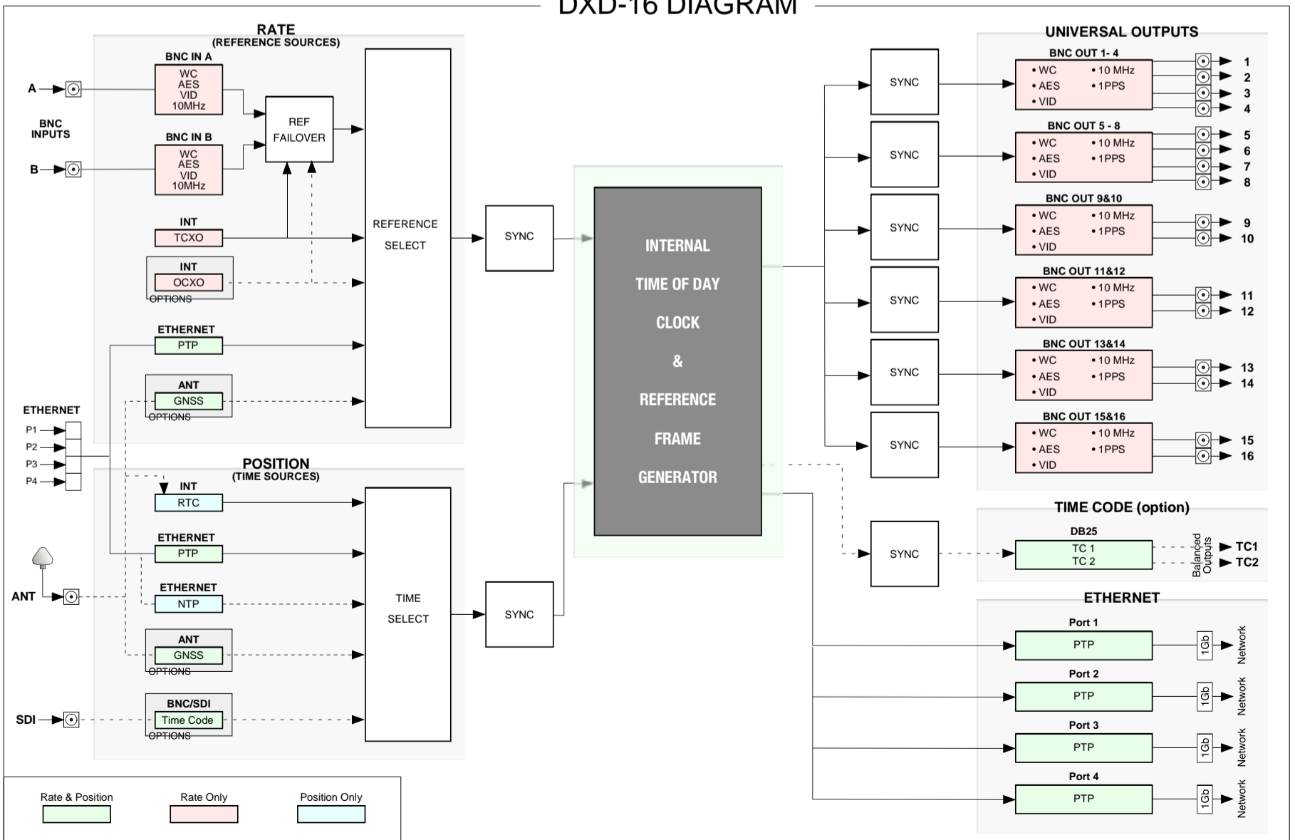
DXD-16 DIAGRAM
